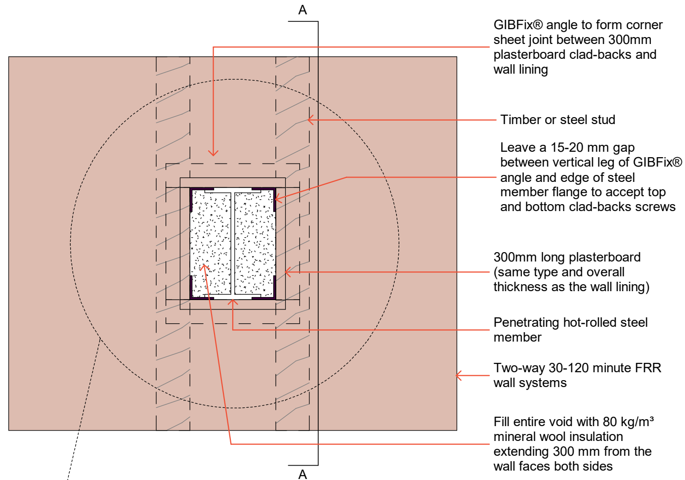
Universal Beam (UB) example
