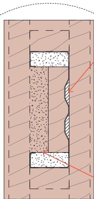
Method 1 (Insulation packing only)
