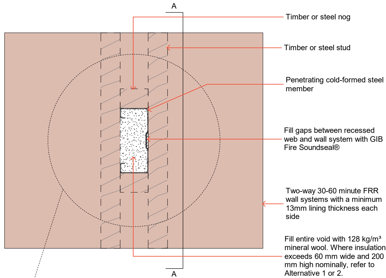
Method 1 (Insulation packing only)
