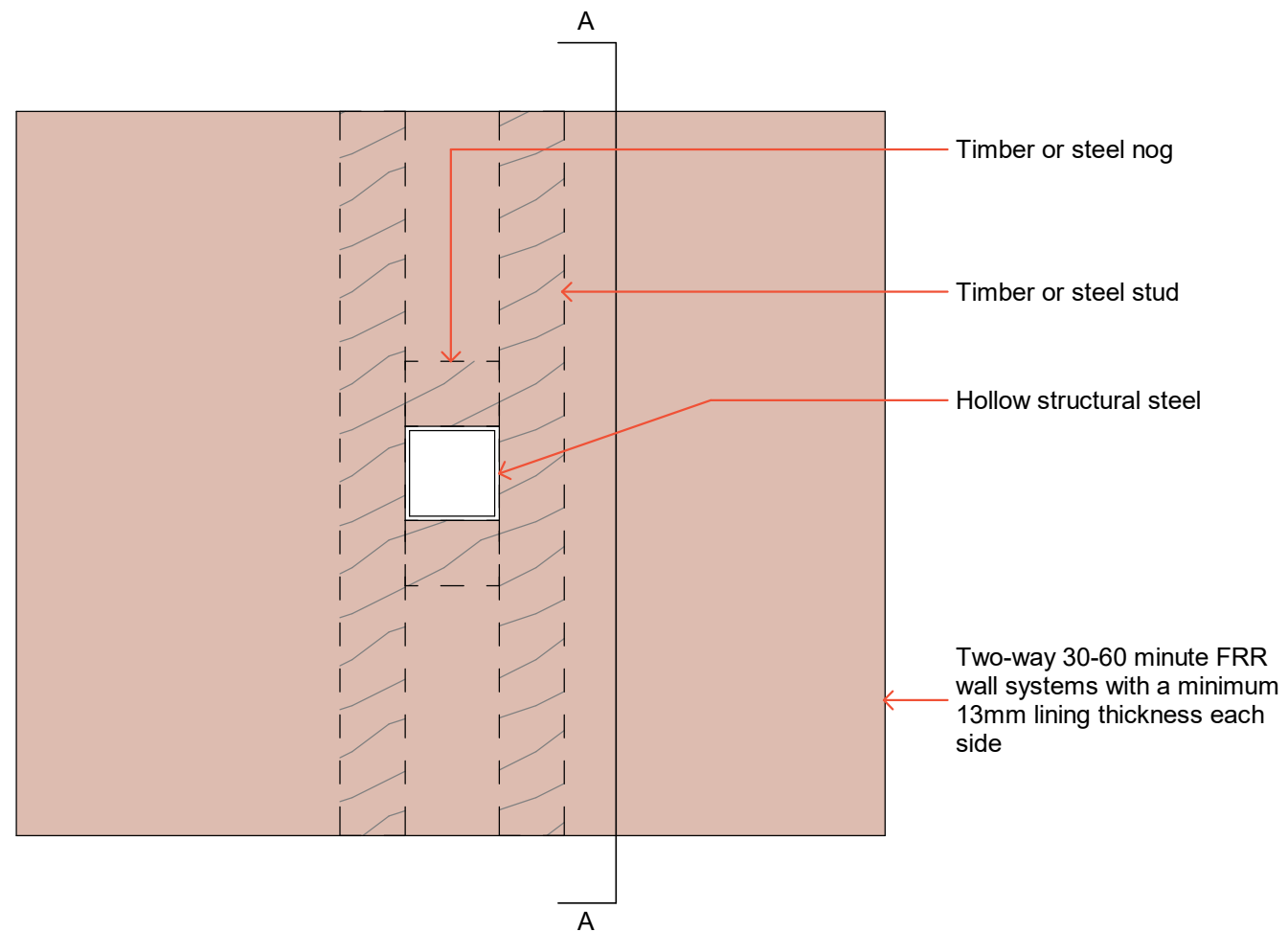
Square Hollow Section (SHS) example
