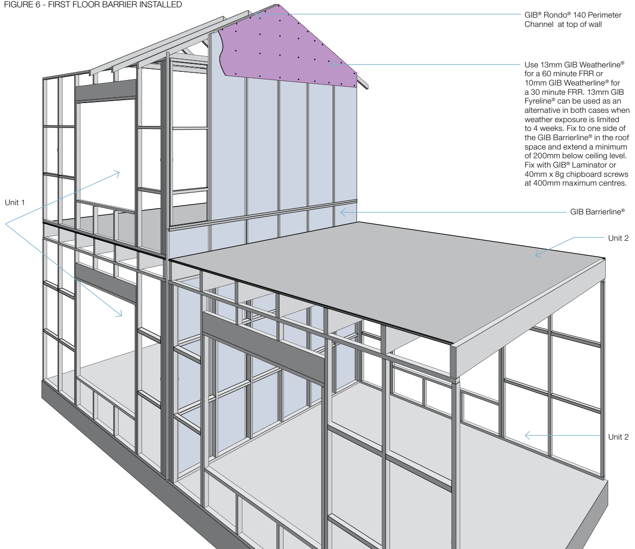
FIGURE 6 - FIRST FLOOR BARRIER INSTALLED
