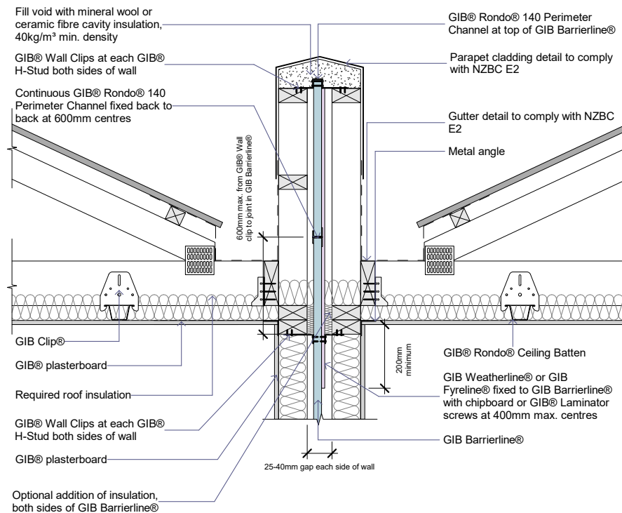
DETAIL AT ROOF/CEILING AND PARAPET (END ELEVATION)
