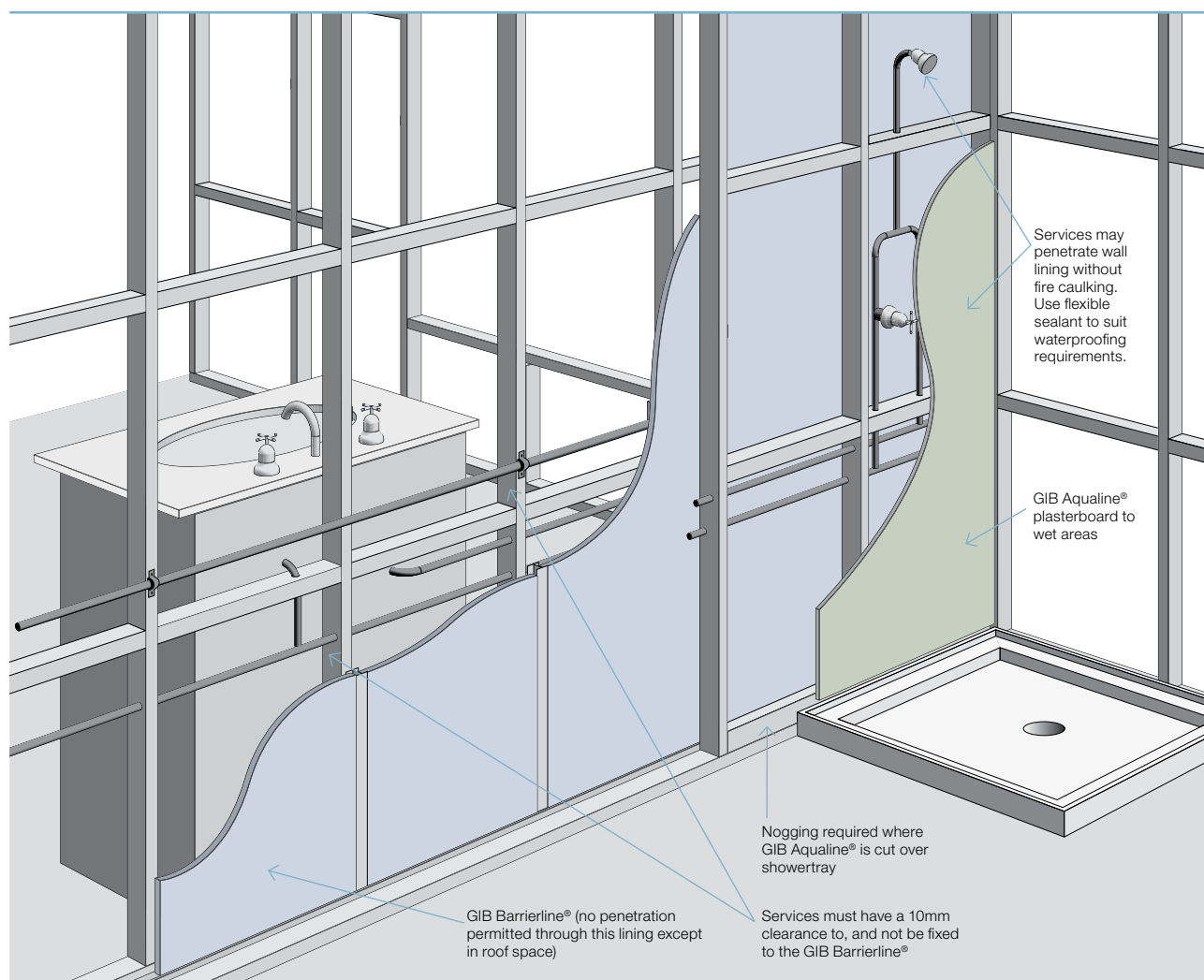
FIGURE 3: TYPICAL PENETRATION FEATURES
