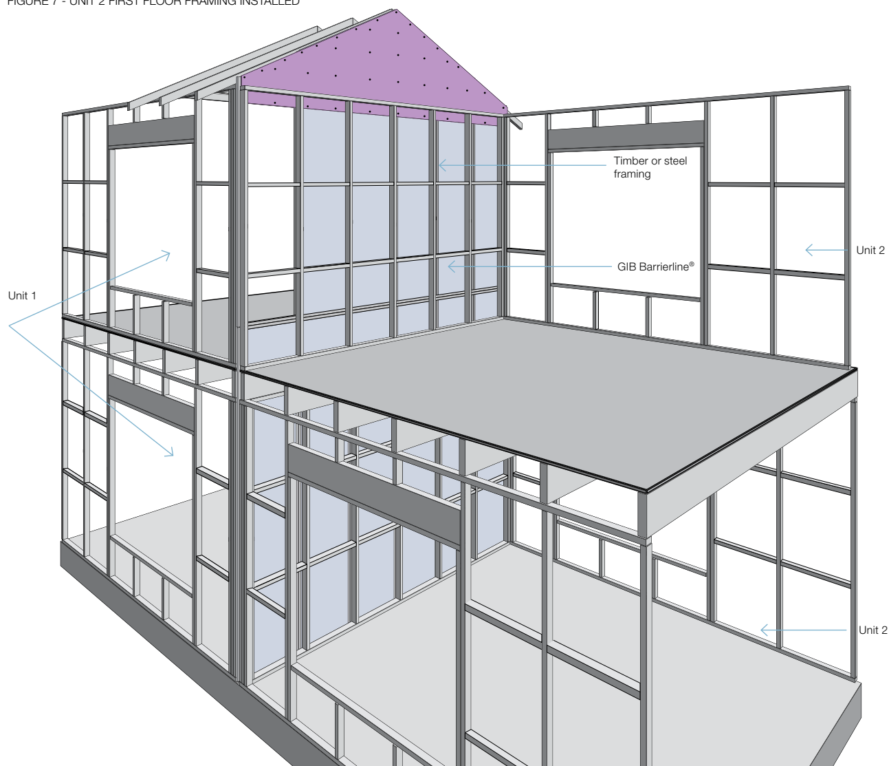
FIGURE 7 - UNIT 2 FIRST FLOOR FRAMING INSTALLED
