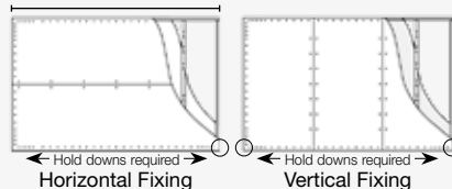
Horizontal Fixing
