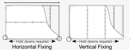
Bracing Element – Plasterboard side shown
