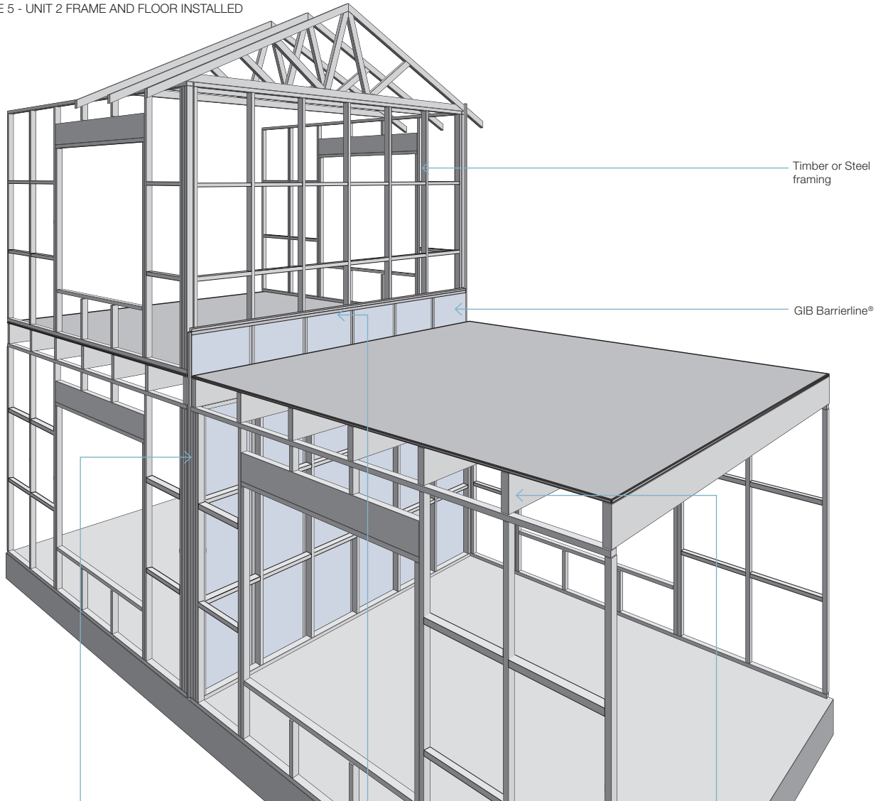
STEP 2 FIGURE 5 - UNIT 2 FRAME AND FLOOR INSTALLED
