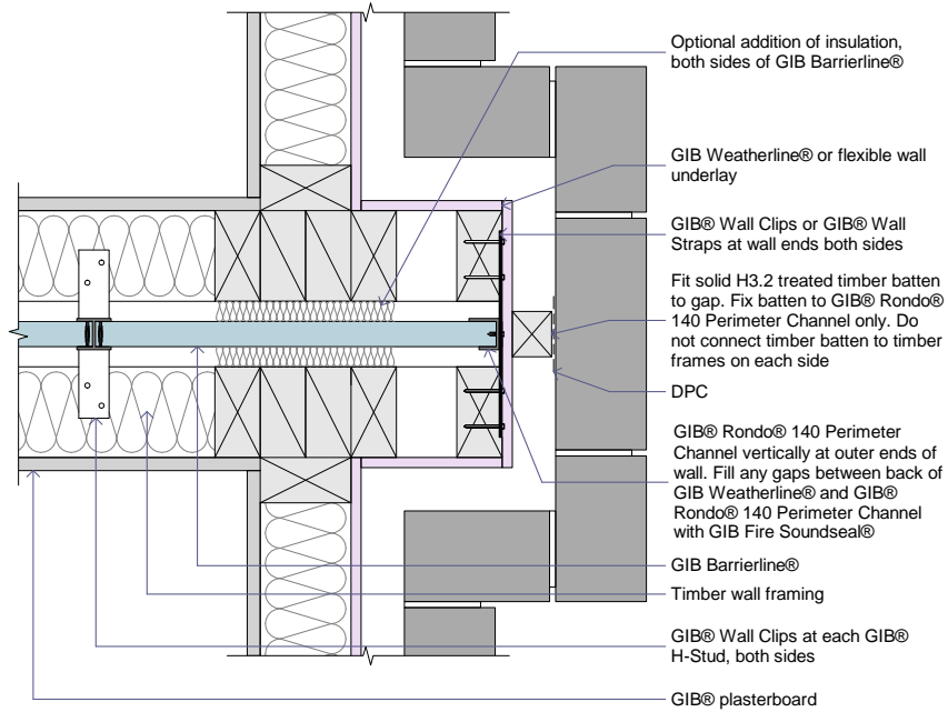
DETAIL AT EXTERNAL BRICK VENEER WALL (WITH GIB WEATHERLINE®)
