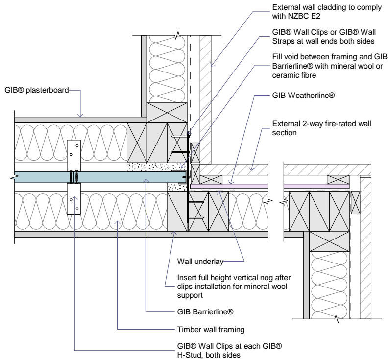
DETAIL AT RETURN IN EXTERNAL TIMBER FRAME WALL (WITH GIB WEATHERLINE®)
