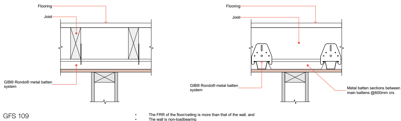
Figure 5: GIB® Rondo® Metal Batten Systems (Section view) - Option 3
