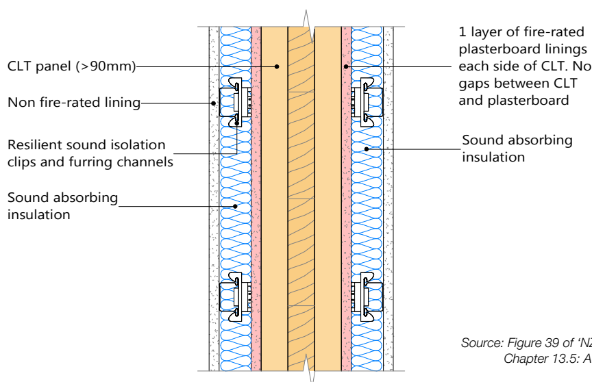
Figure 3: Mass timber wall panel with fire rated wall linings mounted directly on mass timber. Standard wall lining mounted on resilient acoustic clips and furring channels (plan view)
