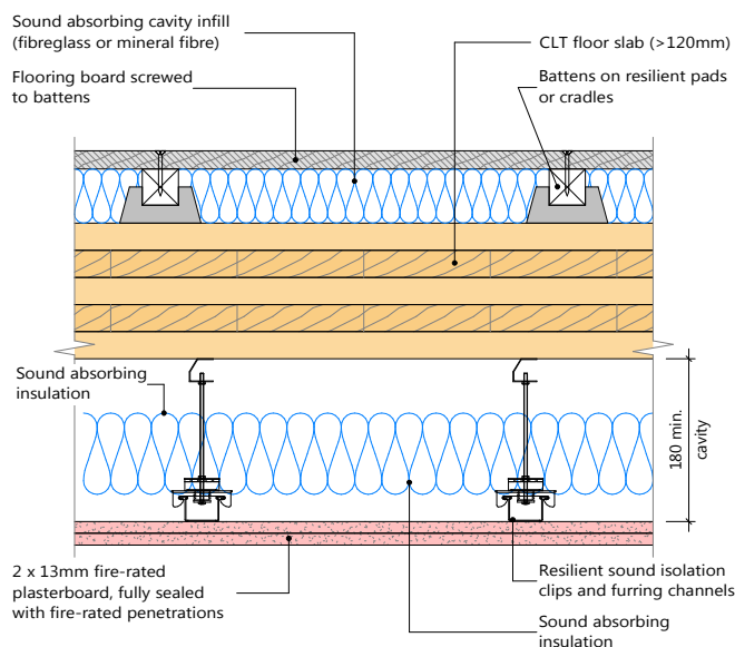
Figure 5: Mass timber floor with a generic lightweight floating floor system – Option 1 (section view)
