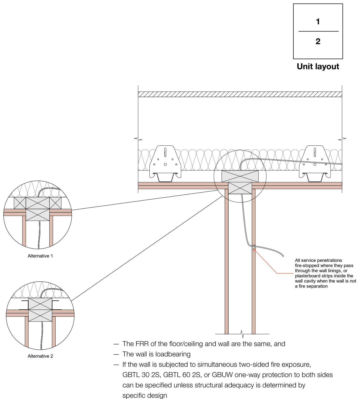
Figure 3: Services within loadbearing wall passing through the top plate at ceiling level
