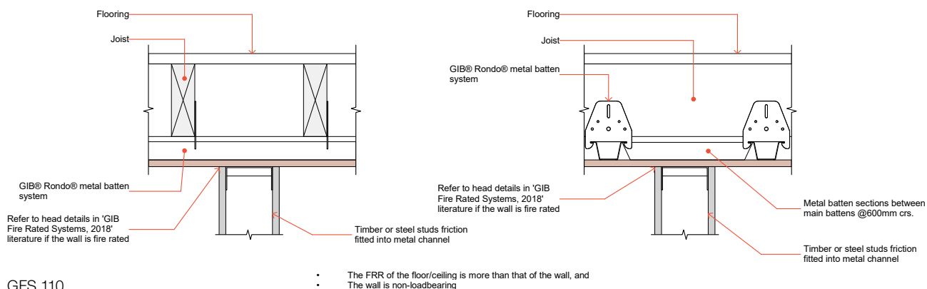
Figure 6: GIB® Rondo® Metal Batten Systems (Section view) - Option 4
