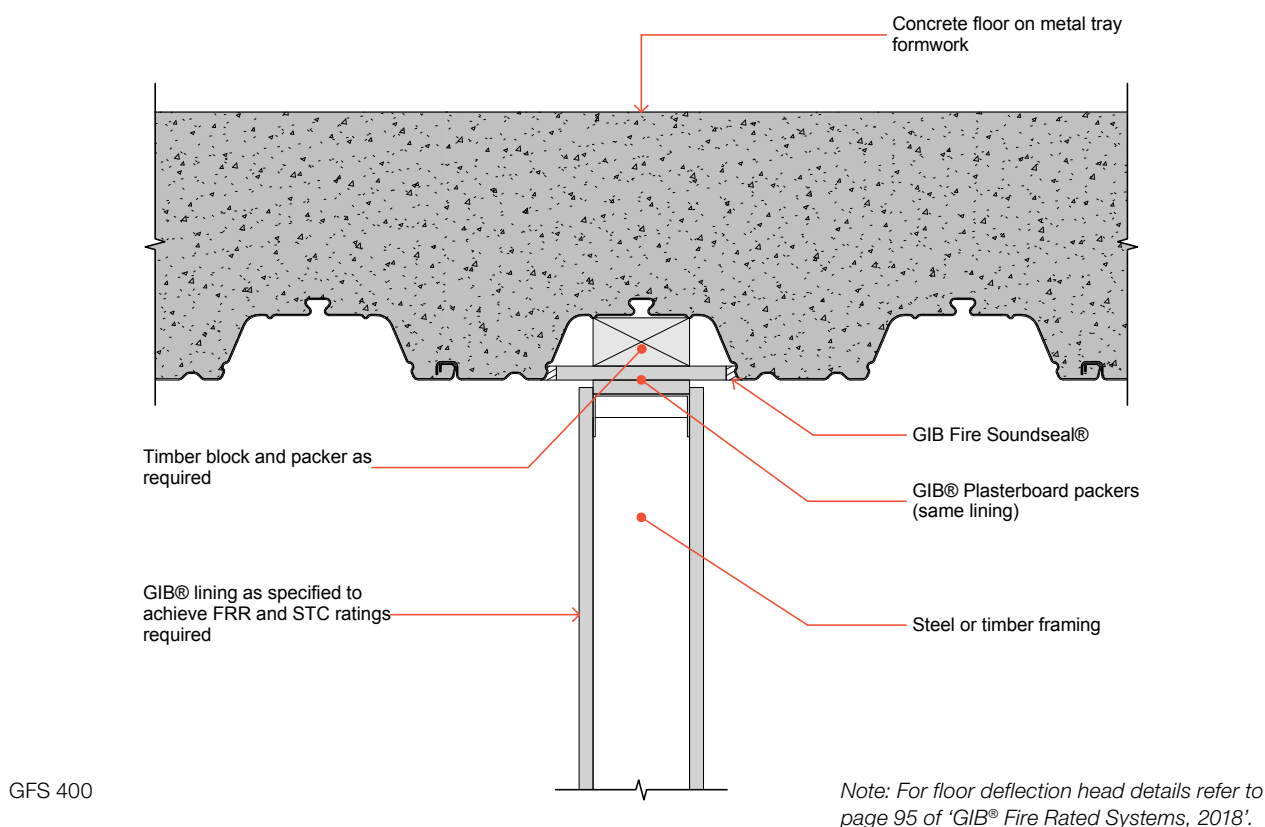
Figure 1: ComFlor® detail for wall with profile – Option 1
