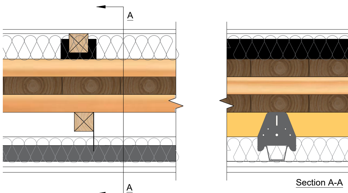
Figure 8: Mass timber floor with two layers of suspended ceiling lining mounted on timber, resilient acoustic clips and furring channels (section view)
