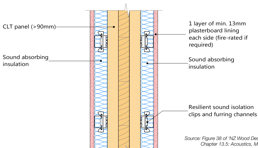
Figure 2: Mass timber wall panel with fire rated wall linings mounted on resilient acoustic clips and furring channels (plan view)
