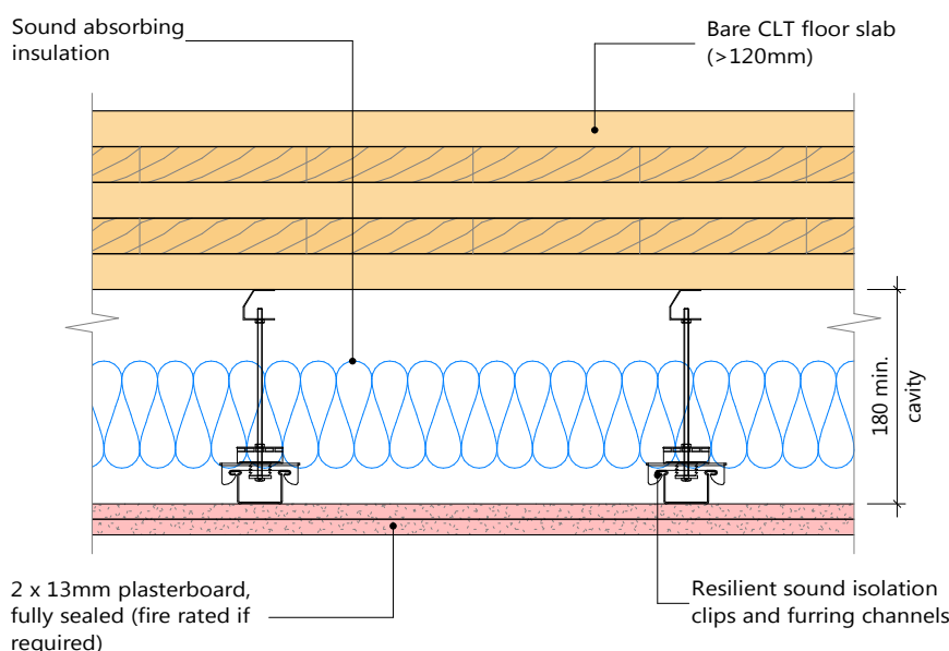
Figure 4: Mass timber floor with resiliently attached suspended ceiling (section view)
