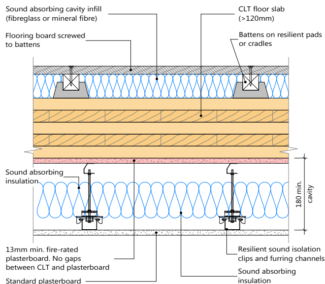
Figure 6: Mass timber floor with a generic lightweight floating floor system – Option 2 (section view)
