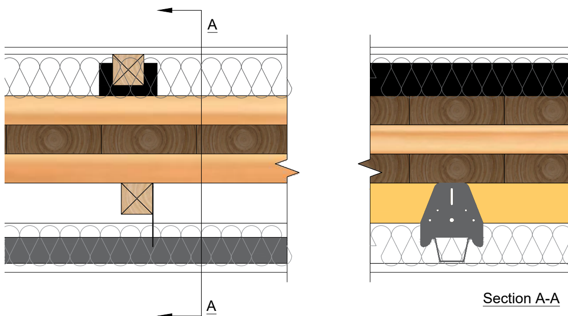
Figure 7: Mass timber floor with a single layer of suspended ceiling lining mounted on timber, resilient acoustic clips and furring channels (section view)
