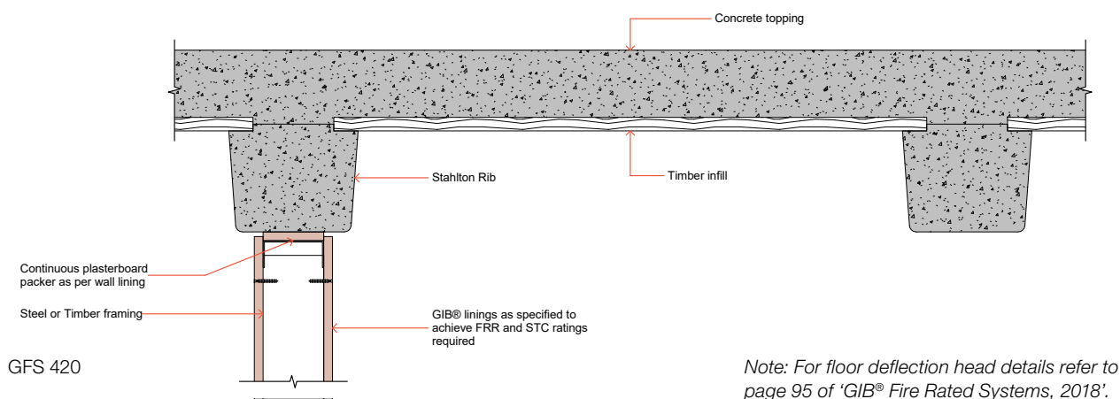
Figure 2: Junction to the underside of timber infill
