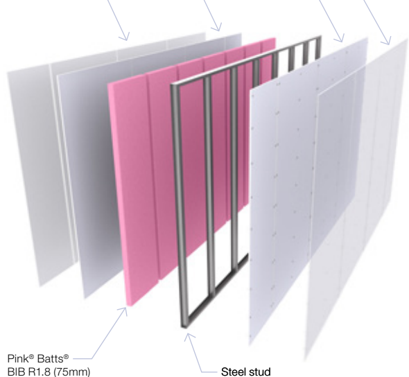
Layers of 10mm or 13mm GIB Braceline®/GIB Noiseline® as prescribed in table above
