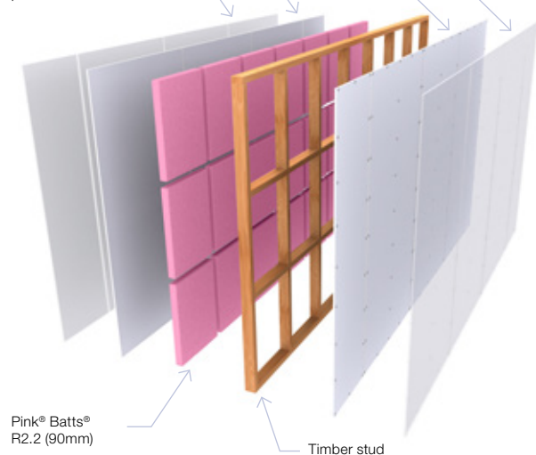
Layers of 10mm or 13mm GIB Braceline®/GIB Noiseline® as prescribed in table above
