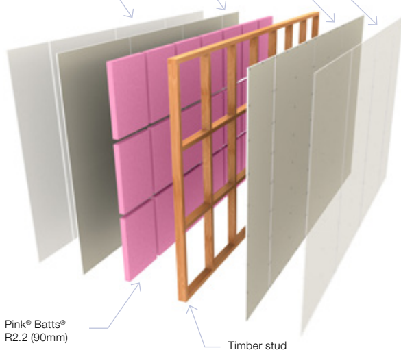
Layers of GIB® Standard Plasterboard as prescribed in table above
